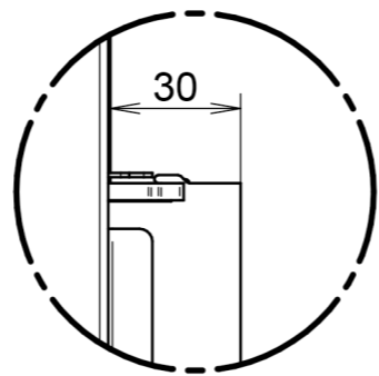
DETAIL A 1:2
